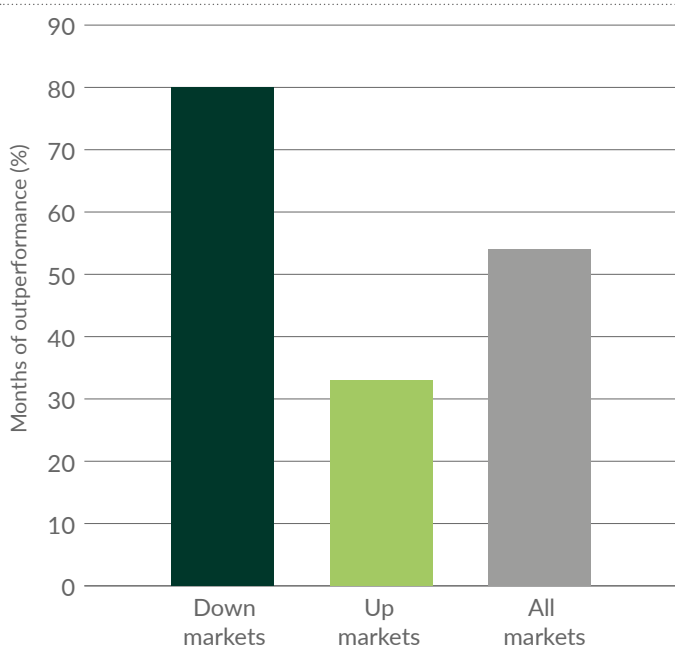
Global Emerging Markets All Cap Investment style - downside protection Composite outperformance (USD net of fees)
