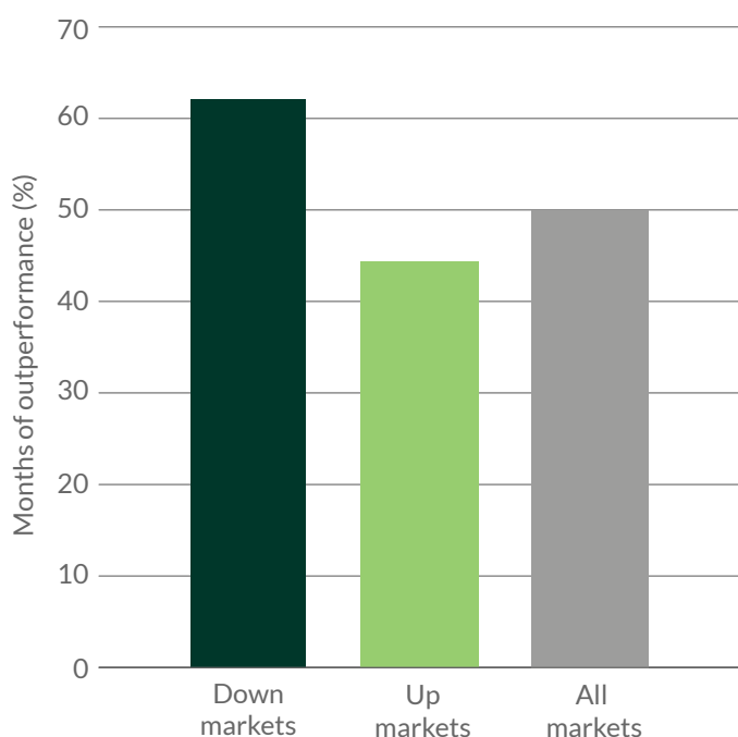
Investment style - downside protection Representative Portfolio outperformance since launch (AUD net of fees)
